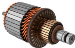
(a) Rotor
